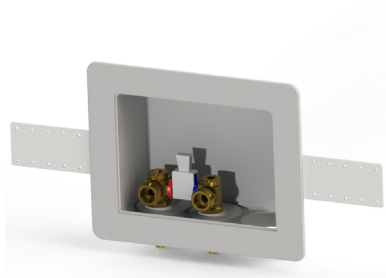
Plastic Switch Hitter™ W/ Plastic Simplex Handle and Crimp PEX Valves OB-435
