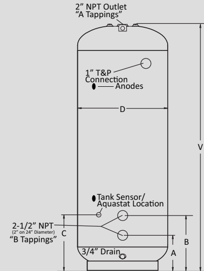
24" & 28" DIAMETER TANKS
