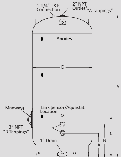
24" & 28" DIAMETER TANKS
